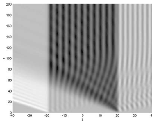
Figure 12: Grayscale plot of the free surface elevation of subcritical flow over a plateau situated at -20 < \xi < 20 . In this calculation, \beta = 0.25 and f = -0.85 . Flow is from left to right.
