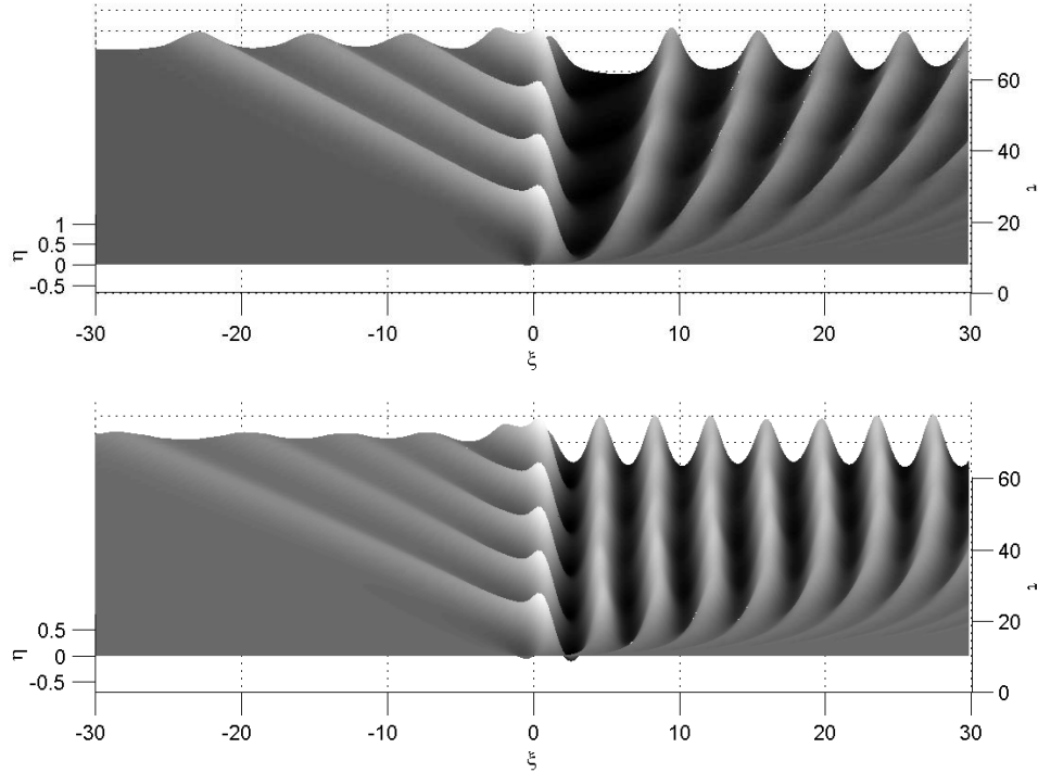
Figure 11: Free surface evolution of a subcritical flow over a hole according to the forced KdV (16) equation with h = -\frac{1}{2}\sqrt{\frac{2}{\pi}}\exp\left(-\frac{x^2}{2}\right) , f = -0.25 (top), f = -0.5 (bottom). Flow is from left to right.
