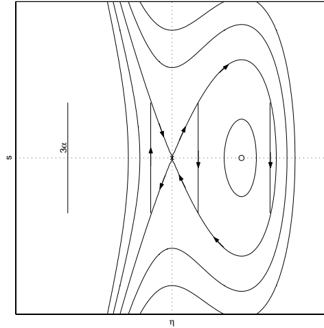
Figure 3: Solutions to the steady problem for f > 0 with Dirac topography h = \alpha\delta(x) . The free-surface has a jump in slope of -3\alpha over the bump. There are two solutions shown for \alpha > 0 and one for \alpha < 0 . Other possible solutions are discussed in the text.
