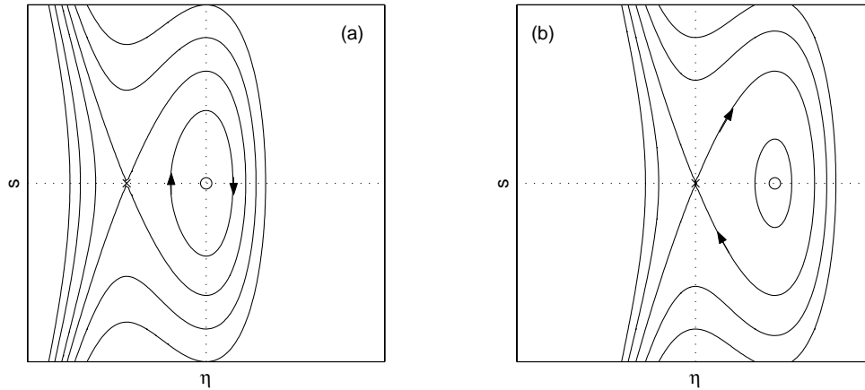
Figure 2: Phase plane of the unforced problem for E = 0 . (a) f < 0 , (b) f > 0 . Circles indicate centers and crosses indicate saddles.
