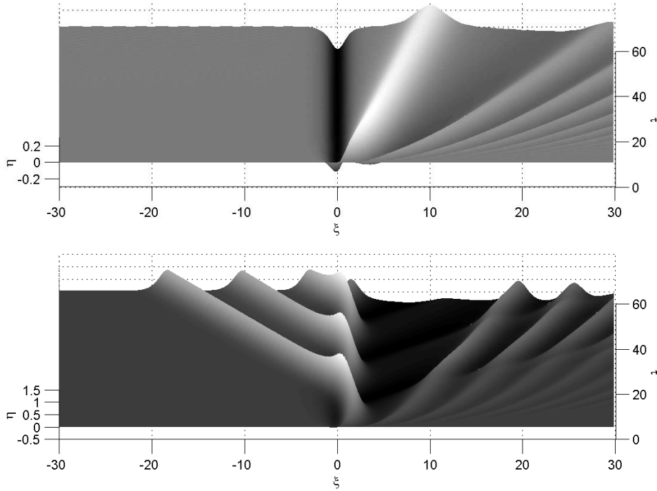
Figure 10: Free surface evolution of a supercritical flow over a hole according to the forced KdV (16) equation with h = -\frac{1}{2}\sqrt{\frac{2}{\pi}}\exp\left(-\frac{x^2}{2}\right) , f = 0.25 (top), f = 0 (bottom). Flow is from left to right.
