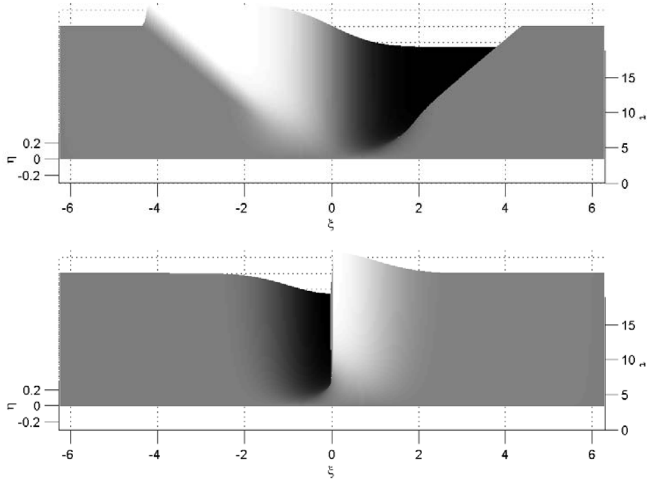
Figure 6: Free surface evolution of a flow over a bump according to the forced Burgers (28) equation for the case \frac{3}{2}\Delta h > f^2 (here f = 0 , \Delta h = 0.1 ). Hydraulic fall over a bump (top) and a shock trapped in a hole (bottom). Flow is from left to right.
