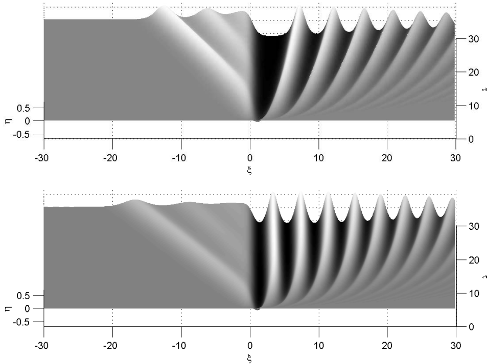
Figure 9: Free surface evolution of a subcritical flow over a bump according to the forced KdV (16) equation with h = \frac{1}{2}\sqrt{\frac{2}{\pi}}\exp\left(-\frac{x^2}{2}\right) , and f = -0.25 (top), f = -0.5 (bottom). Flow is from left to right.
