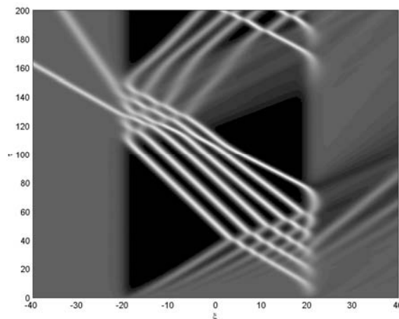
Figure 13: Grayscale plot of the free surface elevation of supercritical flow over a wide valley situated at -20 < \xi < 20 . In this calculation, \beta = -0.25 and f = 0.25 . Flow is from left to right.
