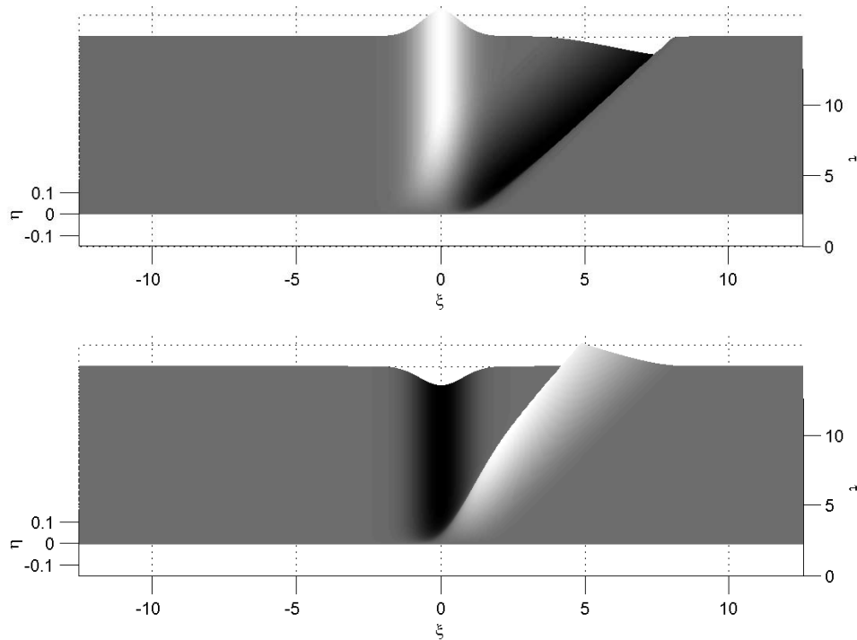
Figure 7: Free surface evolution of a flow over a bump according to the forced Burgers (28) equation for the case \frac{3}{2}\Delta h < f^2 (here f = 0.5 , \Delta h = 0.1 ). Flow over a bump (top) and over a hole (bottom). Flow is from left to right.
