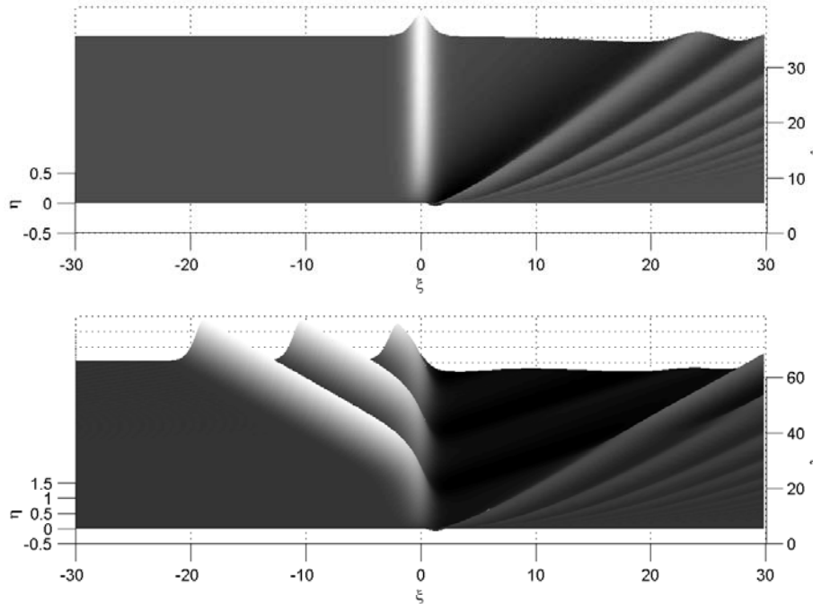
Figure 8: Free surface evolution of a supercritical flow over a bump according to the forced KdV (16) equation with h = \frac{1}{2}\sqrt{\frac{2}{\pi}}\exp\left(-\frac{x^2}{2}\right) , and f = 0.5 (top), f = 0.25 (bottom). Flow is from left to right.
